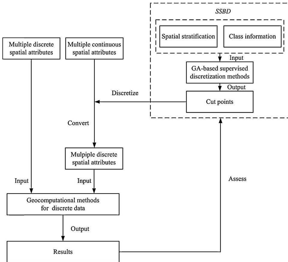
Fig. 2. Flowchart of discretization and assessment process for SSBD.
