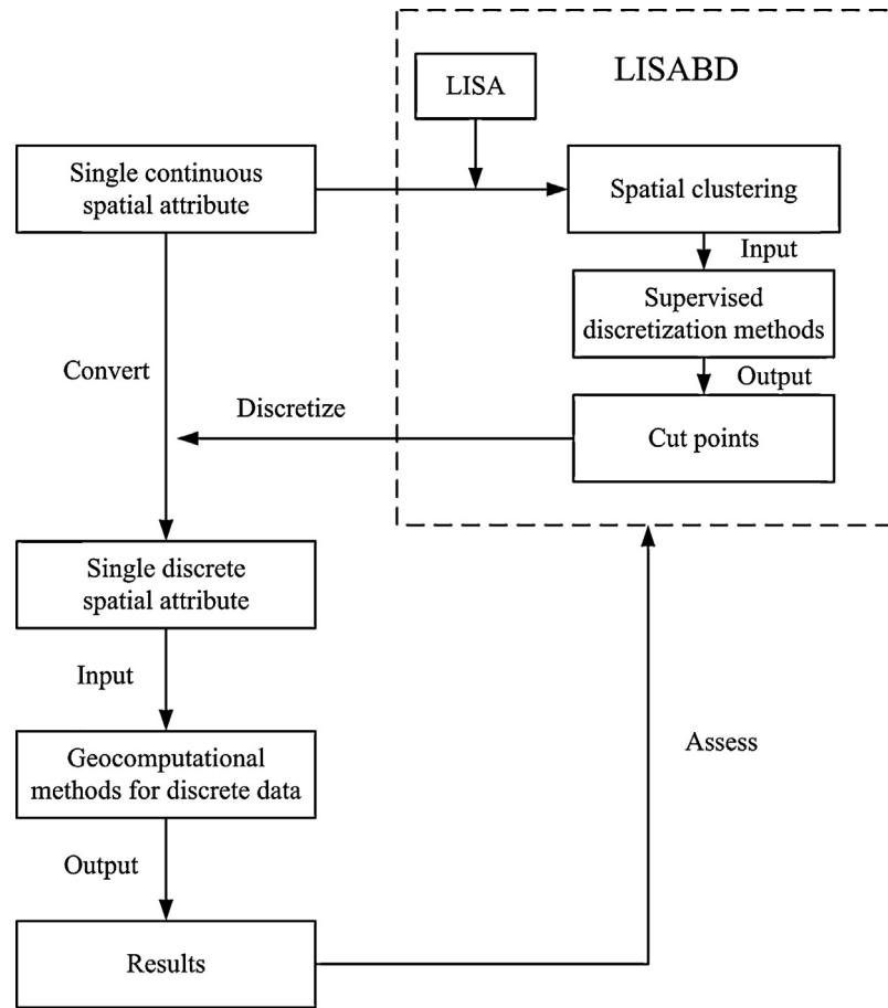
Fig. 1. Flowchart of discretization and assessment process for LISABD.
